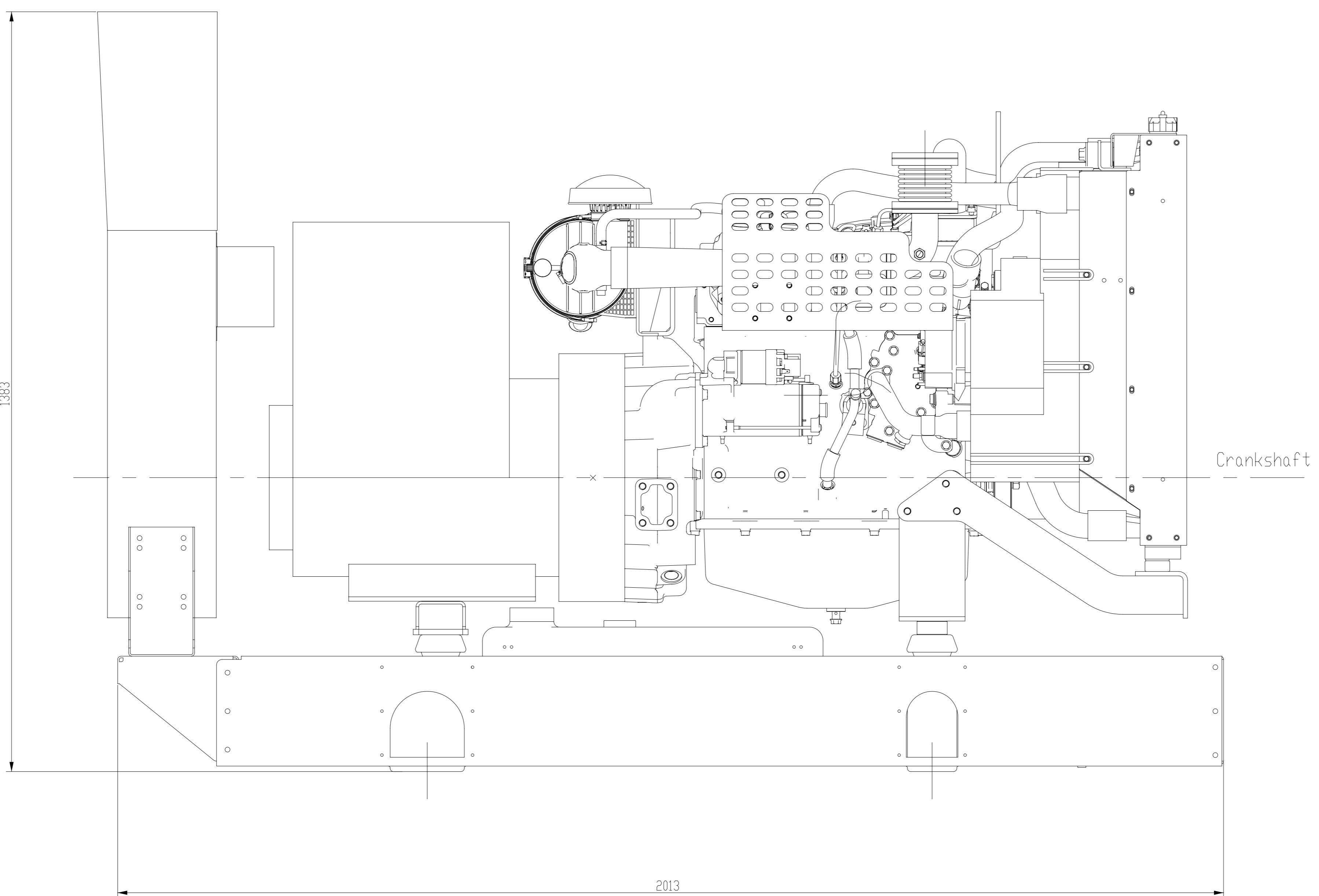
RIGHT VIEW GEF3250MA - 230V only
